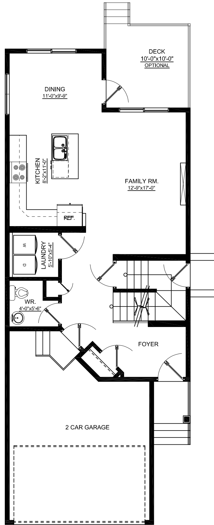
MAIN FLOOR PLAN 746.40 SQ. FT.
