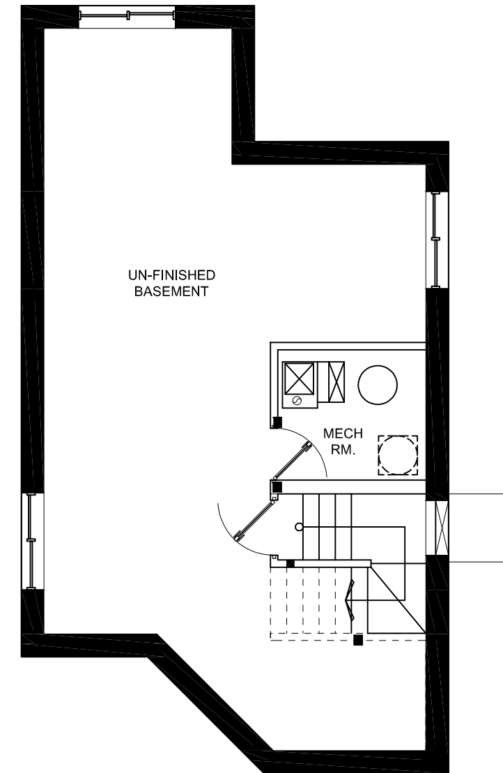
BASEMENT FLOOR PLAN 600 SQ. FT. (NOT INCLUDING MECH RM. & STAIRS)
